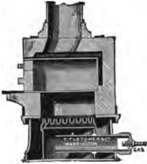
FIG. 25.—Muffle furnace.
